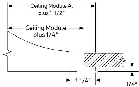
Frame Type SFM (Surface Mount) Full Face
