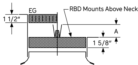
Model EG Equalizing Grid
