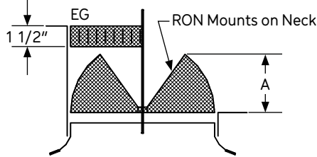
Model EG Equalizing Grid
