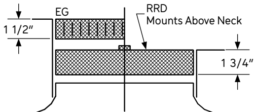
Model EG Equalizing Grid
