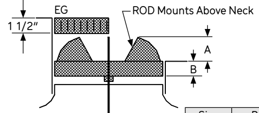
Model EG Equalizing Grid
