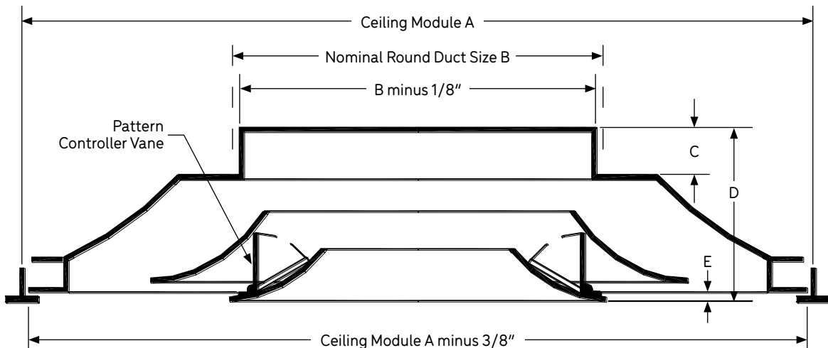
Border Type LTF (Lay-In) Full Face.
