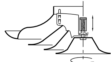
Type 3: Rotating (available in neck sizes 6"-36")
