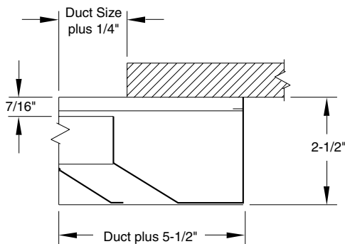
SF - SURFACE MOUNT DETAILS
