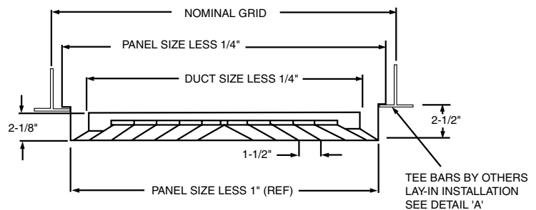
LAY-IN T-BAR DETAILS
