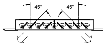
Adjustable Blade Detail
