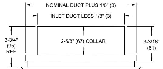
SRSS (Square to Round) Detail
