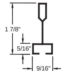
Narrow T-bar Detail (All narrow Tees provided by others)
