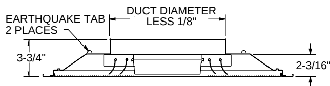
Side View Detail, SF Frame
