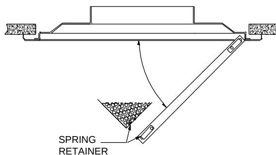
Face Hinge Detail
