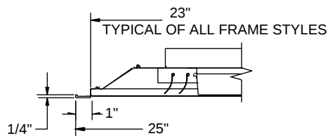
Frame SF (Surface Mount) *minimum ceiling opening 23-1/4"
