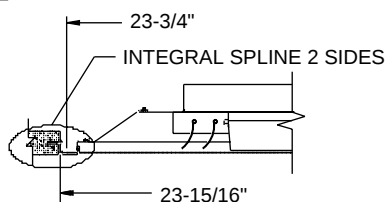
Frame PL (Spline)
