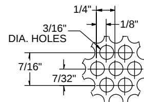
Perforated Pattern Detail (51% free area)
