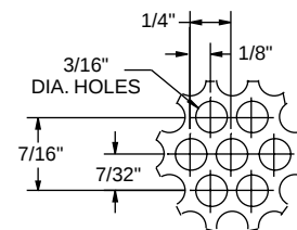
Perforated Pattern Detail (51% free area)
