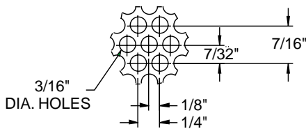
Perforated Pattern Detail (51% free area)
