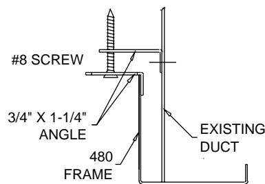
Concealed Fastening (not available with SOBD)
