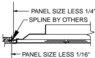
Frame PL (Spline)
