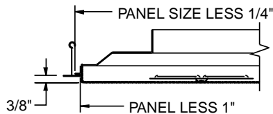
Frame TG** (Tegular)
