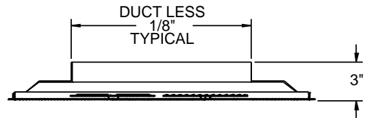
Side View Detail, LT Frame
