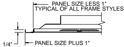
Frame SF (Surface Mount) *minimum ceiling opening 23-1/4"
