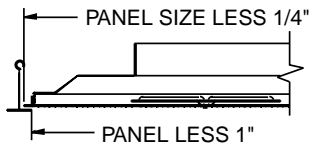
Frame LT (Lay-in T-Bar)
