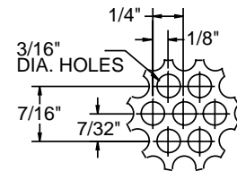
Perforated Pattern Detail (51% free area)
