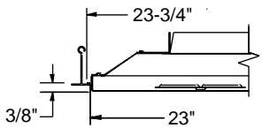
Frame TG** (Tegular)
