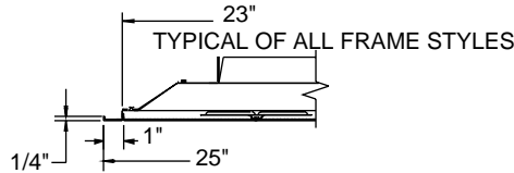
Frame SF (SurFace Mount) *minimum ceiling opening 23-1/4"
