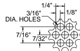
Perforated Pattern Detail (51% free area)
