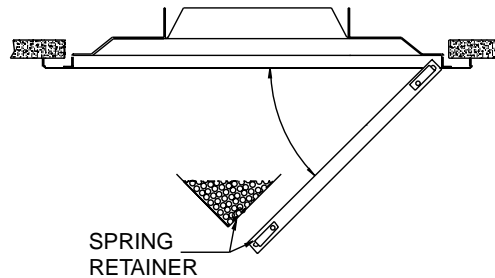
Face Hinge Detail
