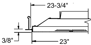
Frame TG** (Tegular)
