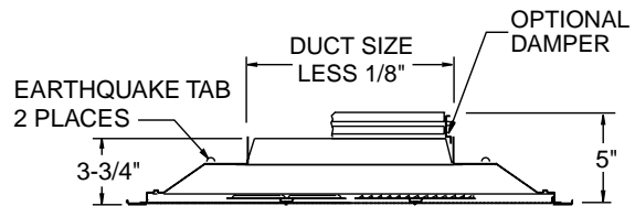
Side View/Damper Detail, SF Frame
