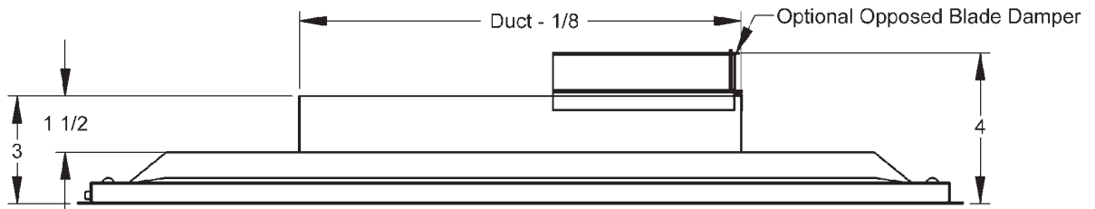
Side View/Damper Detail Square Neck
