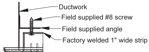
Concealed Mounting Detail
