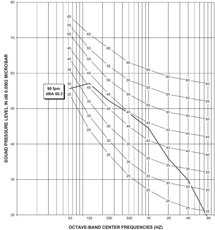
48x24 PSC (Motor) Sound 30" FROM FILTER FACE
