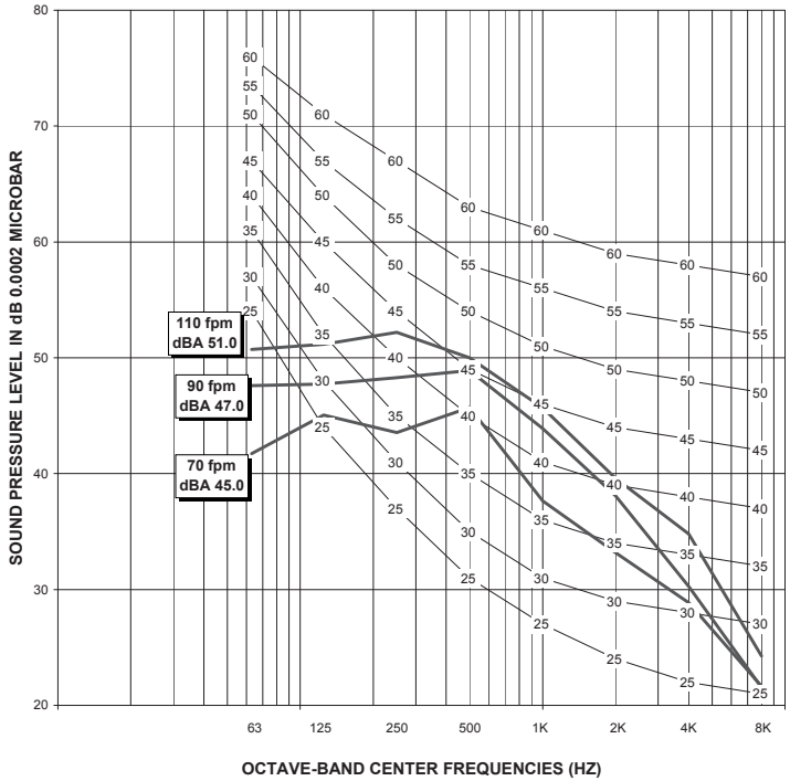
24x24 ECM Option Sound 30" FROM FILTER FACE
