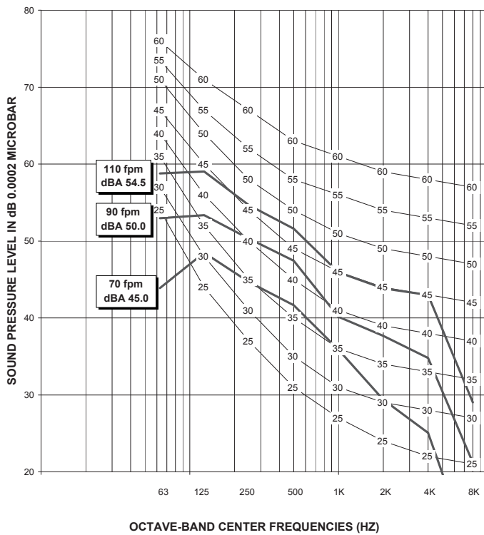
48x24 ECM Option Sound 30" FROM FILTER FACE
